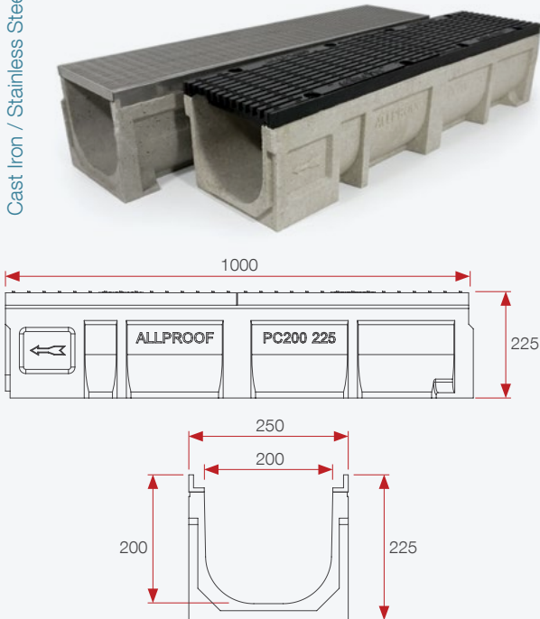
200mm Clear Opening Inline Sump Cast Iron / Stainless Steel
