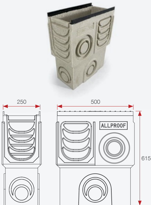
200mm Clear Opening Inline Sump Cast Iron / Stainless Steel
